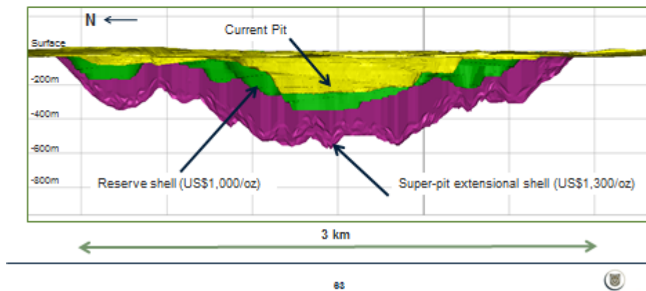
Damang Super-pit Conceptual Shell
